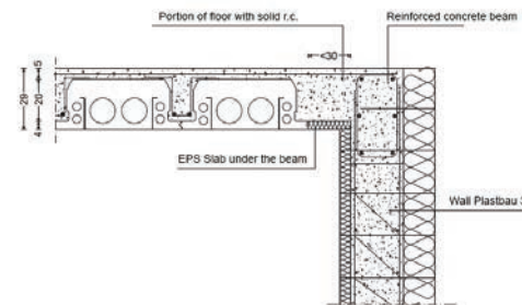
Section Y-Y
